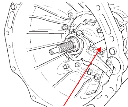
Fork Shaft
