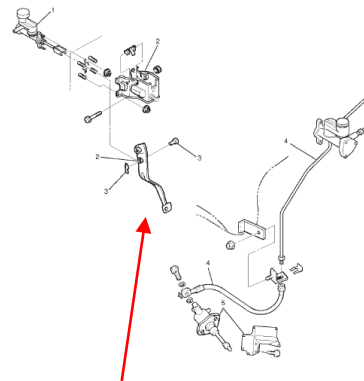
Pedal Bushings & Hydraulics
